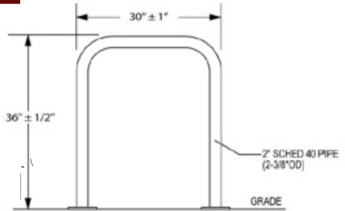
ELEVATION VIEW 1 HOOP - 2 BIKE CAPACITY
